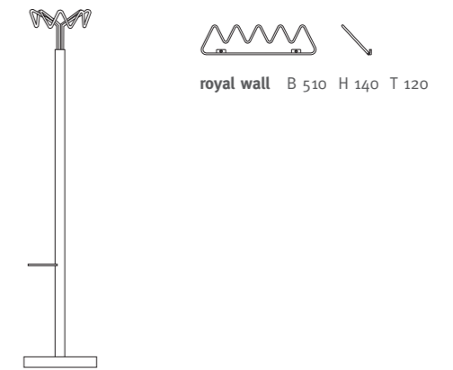
royal wall B 510 H 140 T 120 royal D 350 H 1735
