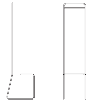
chair B 400 H 1695 T 490 ST 250
